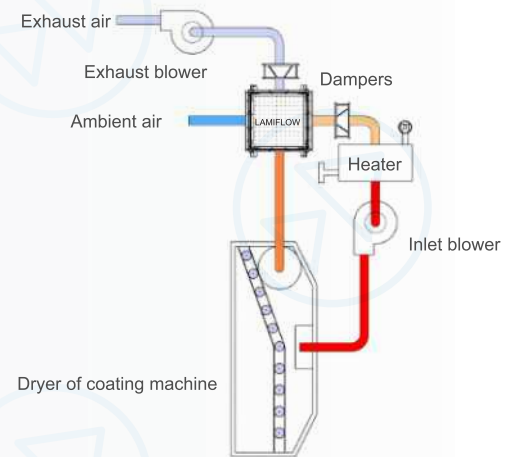
New drying process with Lamiflow heat recovery
