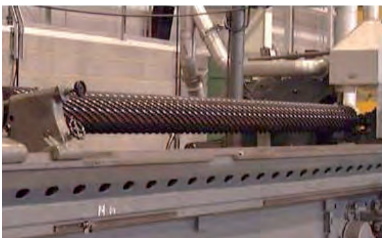
Cylinder Grinding
