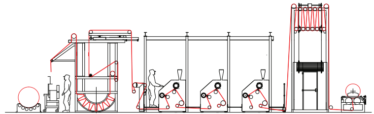
Off-Line Shear
