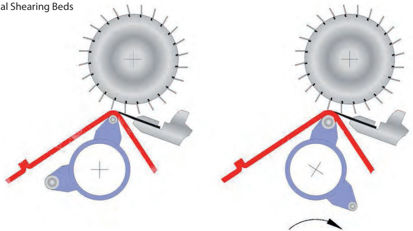
Dual Shearing Beds
