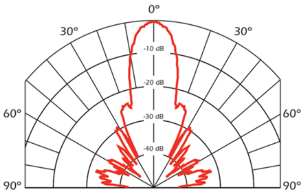
Figure 18. Directivity pattern of the LS-200
