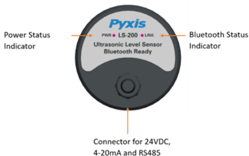
Figure 3. Sensor connection and indicators
