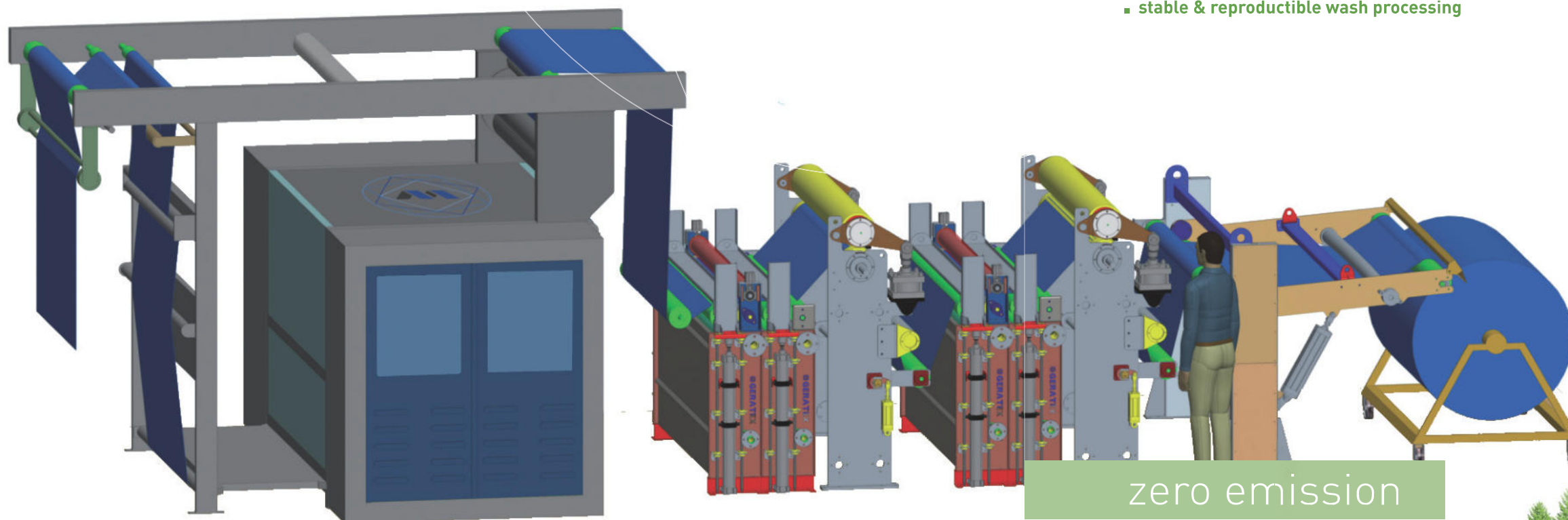
diamond denim finishing® processing line
